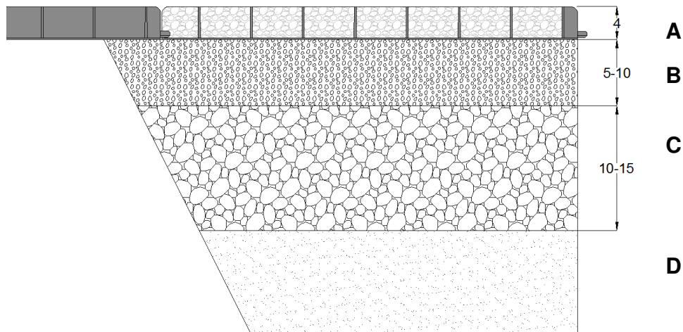
A- Salvaverde B; B- Bedding layer; C- Foundation; D- Natural soil
