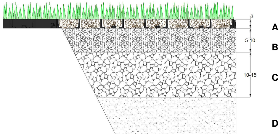
A- Runfloor F03; B- Couche de pose; C- Couche portante; D- Sol existant
