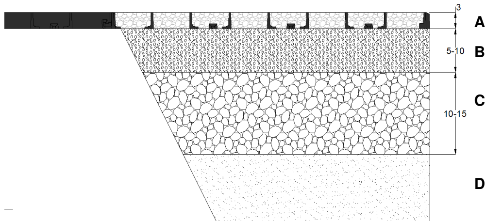
A- Runfloor F03; B- Couche de pose; C- Couche portante; D- Sol existant
