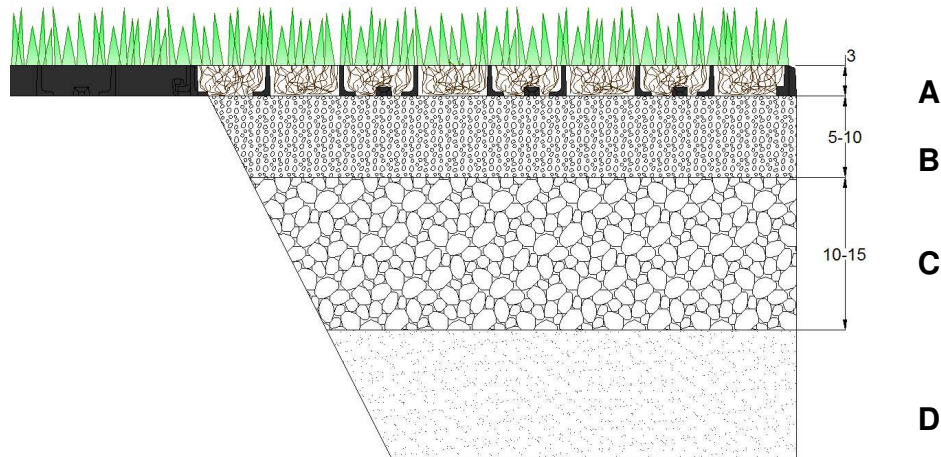
A- Runfloor F05; B- Couche de pose; C- Couche portante; D- Sol existant
