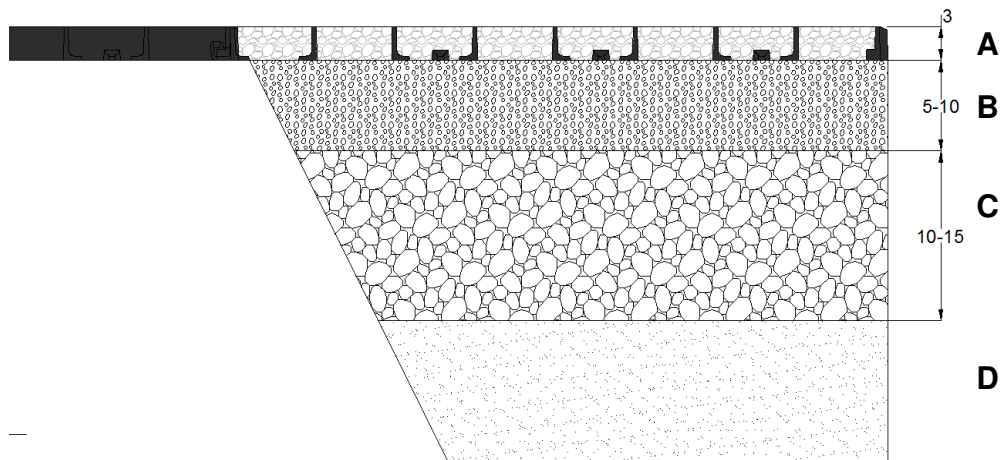
A- Runfloor F04; B- Bedding layer; C- Foundation; D- Natural soil
