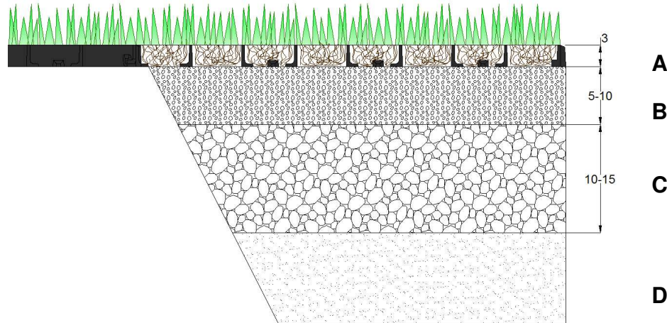
A- Runfloor F04; B- Bedding layer; C- Foundation; D- Natural soil
