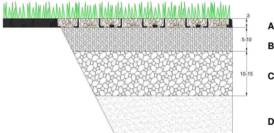
A- Runfloor F05; B- Bedding layer; C- Foundation; D- Natural soil
