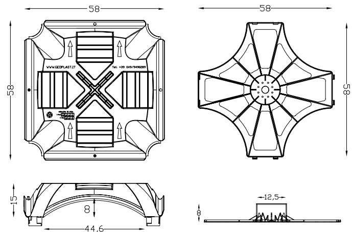
Fig. 1: Shaft and base of the dimensional drawings NEW ELEVATOR
