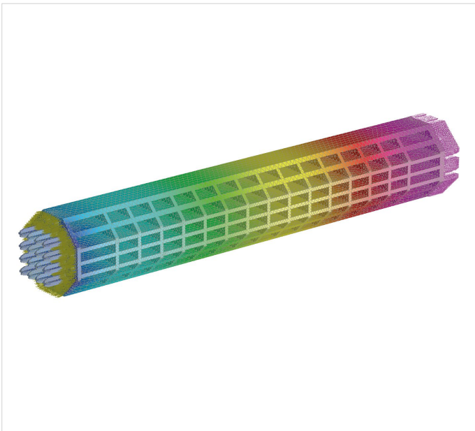
Deformation analysis of new product FEM model
