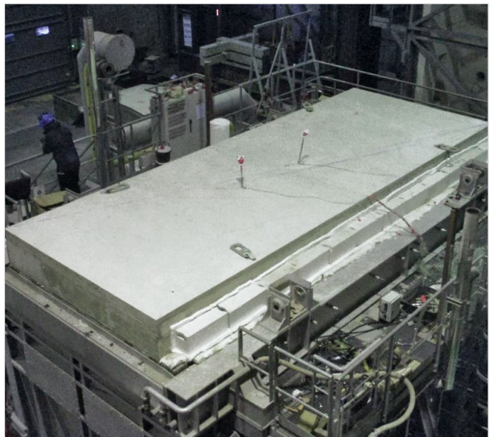
Fire test
